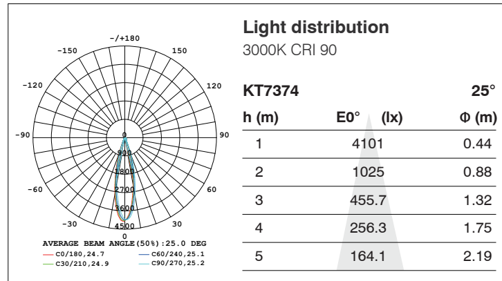
KT7374, 10W, 1027LM
