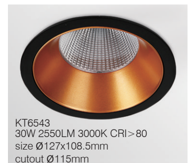
KT6748 10W 660LM 3000K CRI>80 size Ø102x75mm cutout Ø75mm
