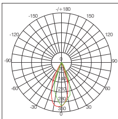
SL368-3W-3000K-40°
