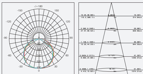
KF1030-25W-3000K-115°
