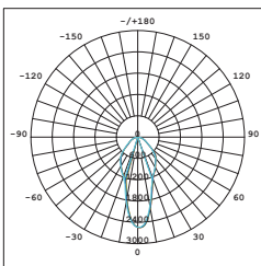
KF1015-40W-3000K-110°
