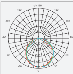
KF1032A-30W-3000K-110°
